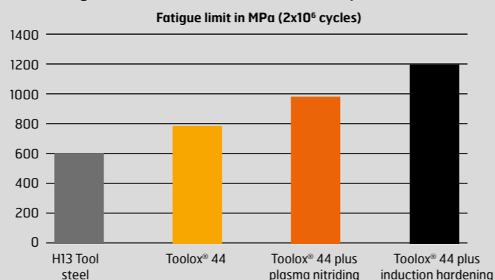
Fatigue limit for Toolox® 44 as tested by SWERIM
